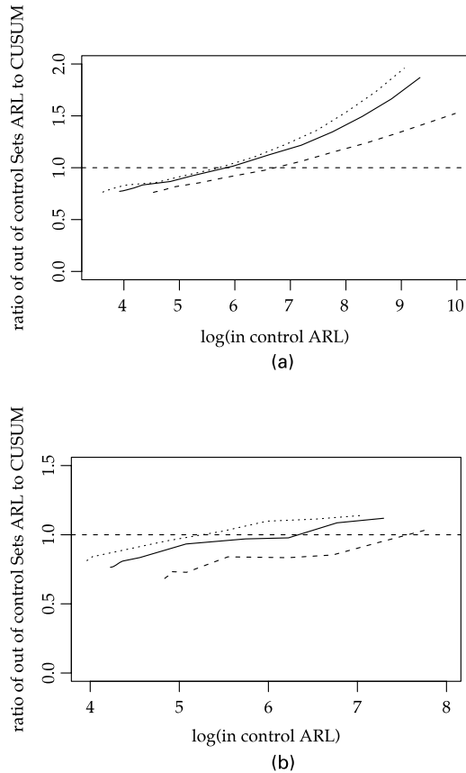
Fig. 6. Ratio of out-of-control ARL for the sets method to that of the CUSUM for fixed log(in-control ARL) (—, \lambda = 1 ; - - - - - , \lambda = 0.5 ; ······, \lambda = 1.5 ): (a) charts testing for a doubling in odds; (b) charts testing for a fivefold increase in odds
