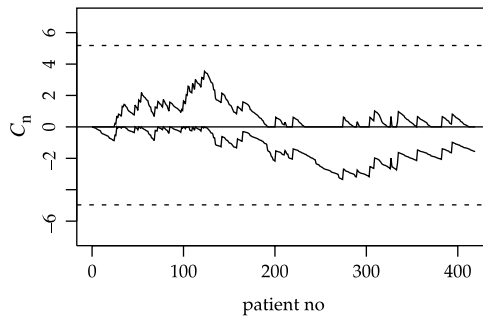
Fig. 7. Two-sided risk-adjusted CUSUM with h_u = 5.18 , h_l = -4.96 and in-control ARL 6700 patients (example 1 data)
