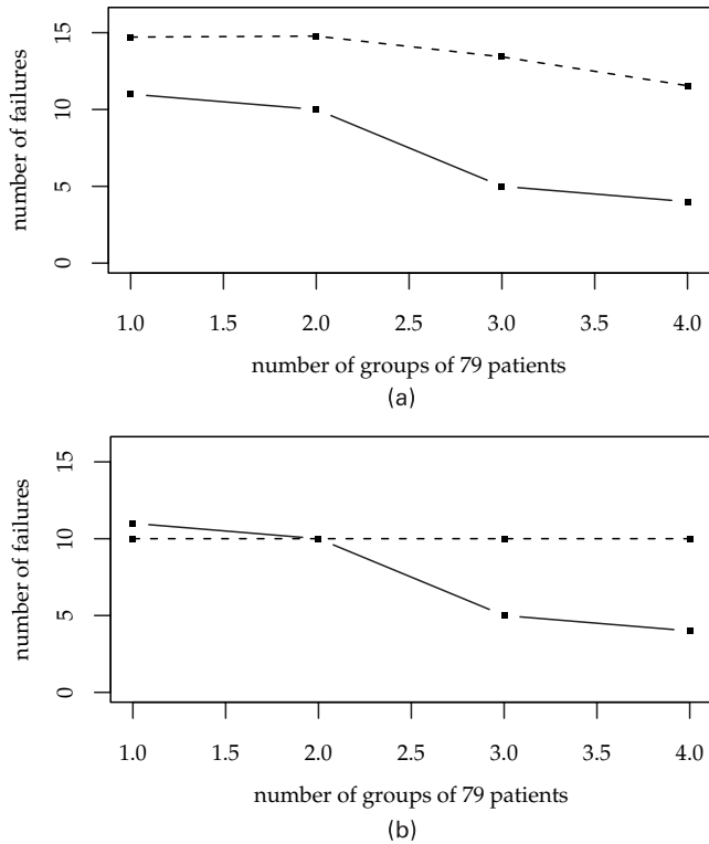
Fig. 4. 6-monthly Shewhart charts testing for a doubling in the odds of 30-day mortality following cardiac surgery (in-control ARL, 84 6-monthly periods): (a) adjusted; (b) unadjusted
