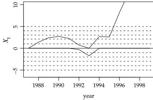
Fig. 8. CUSUM monitoring death-rates per year under Harold Shipman, 1987–1998
